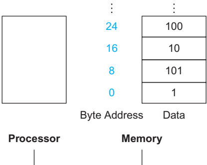
FIGURE 2.3 Actual RISC-V memory addresses and contents of memory for those doublewords. The changed addresses are highlighted to contrast with Figure 2.2 . Since RISC-V addresses each byte, doubleword addresses are multiples of 8: there are 8 bytes in a doubleword.
