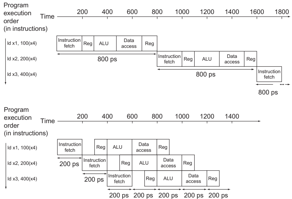
FIGURE 4.25 Single-cycle, nonpipelined execution (top) versus pipelined execution (bottom). Both use the same hardware components, whose time is listed in Figure 4.24. In this case, we see a fourfold speed-up on average time between instructions, from 800 ps down to 200 ps. Compare this figure to Figure 4.23. For the laundry, we assumed all stages were equal. If the dryer were slowest, then the dryer stage would set the stage time. The pipeline stage times of a computer are also limited by the slowest resource, either the ALU operation or the memory access. We assume the write to the register file occurs in the first half of the clock cycle and the read from the register file occurs in the second half. We use this assumption throughout this chapter.
