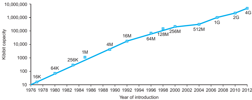
FIGURE 1.11 Growth of capacity per DRAM chip over time. The y-axis is measured in kibibits ( 2^{10} bits). The DRAM industry quadrupled capacity almost every three years, a 60% increase per year, for 20 years. In recent years, the rate has slowed down and is somewhat closer to doubling every two to three years.
